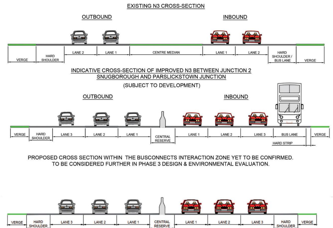
Figure 3: Emerging Preferred Option - Median Widening between Junction 2 Snugborough and Parslicktown Junction
