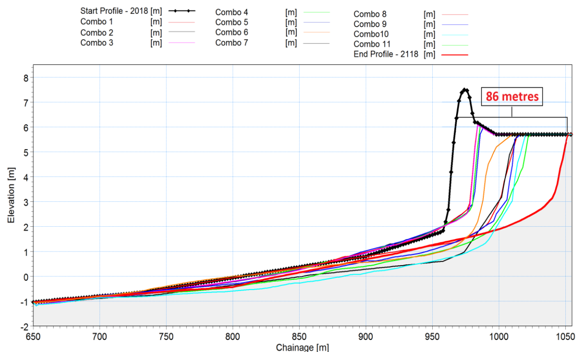
Figure 5.4: The evolution of the beach dune profile at Portrane following the first 11 storm combination events and the final position of the profile by 2118.
