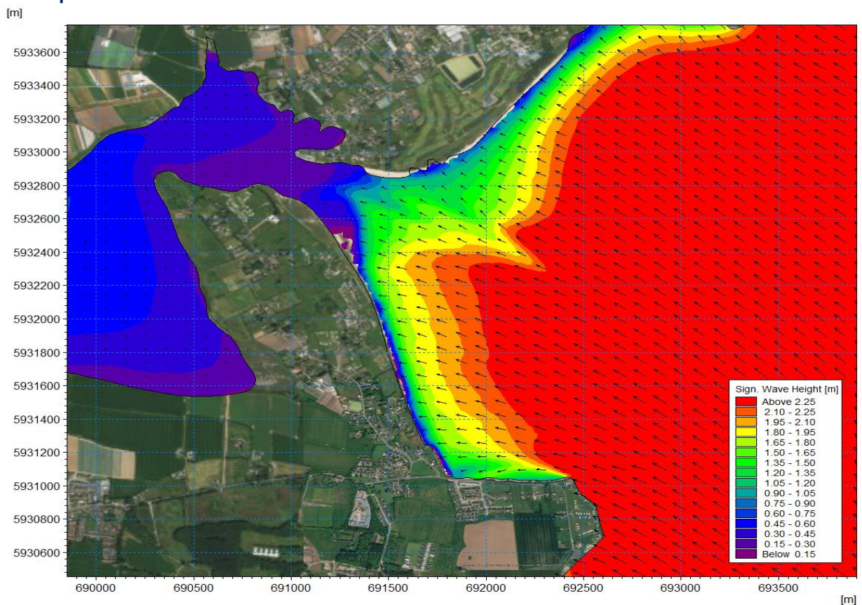
Figure 5.2: Significant wave height and mean wave direction during a joint probability 1 in 200 year return period storm event from the South East.
