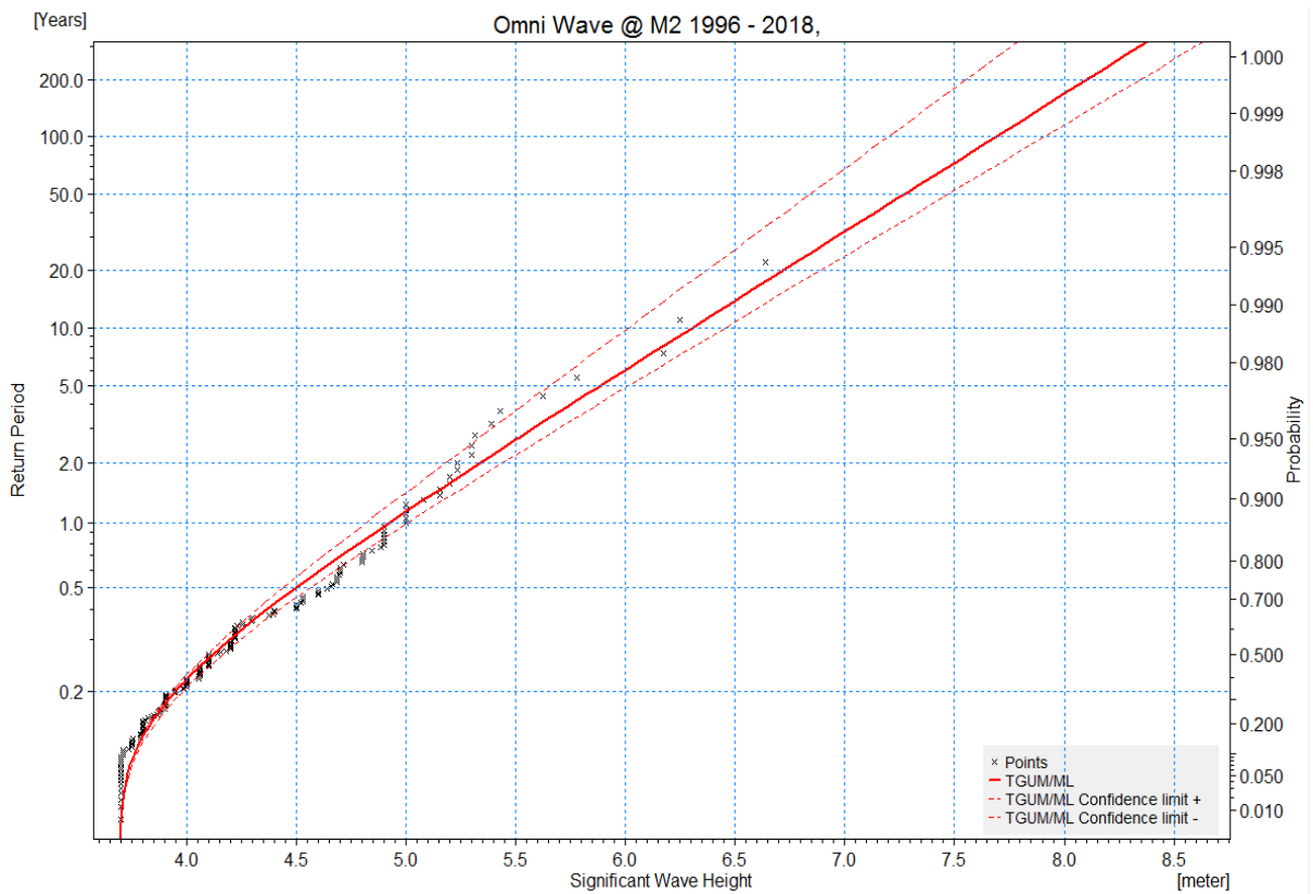
Figure 3.5: Extreme event analysis of offshore waves from all directions between 1996 and 2018.
