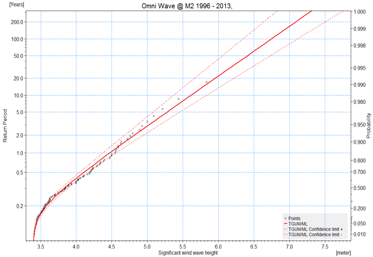
Figure 3.4: Extreme event analysis of offshore waves from all directions between 1996 and 2013.
