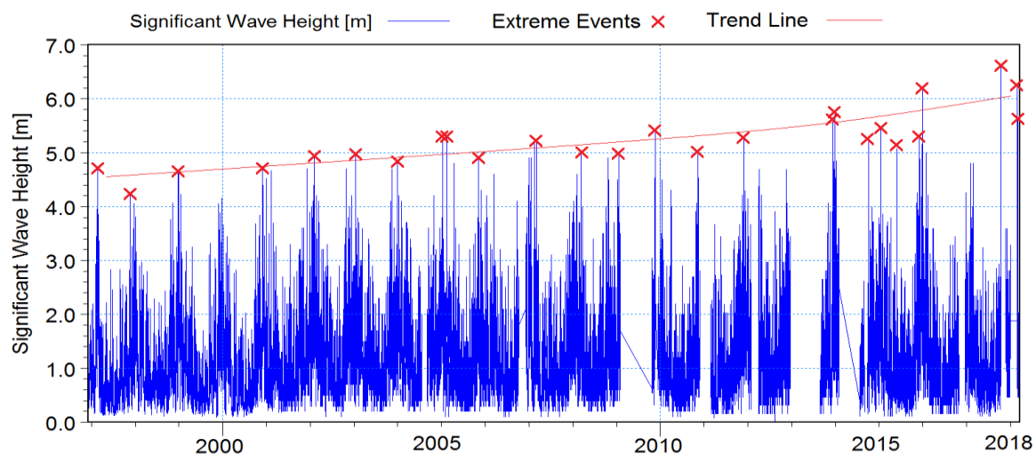
Figure 3.2: Significant wave heights from all wave directions at the M2 buoy between 1996 and 2018.
