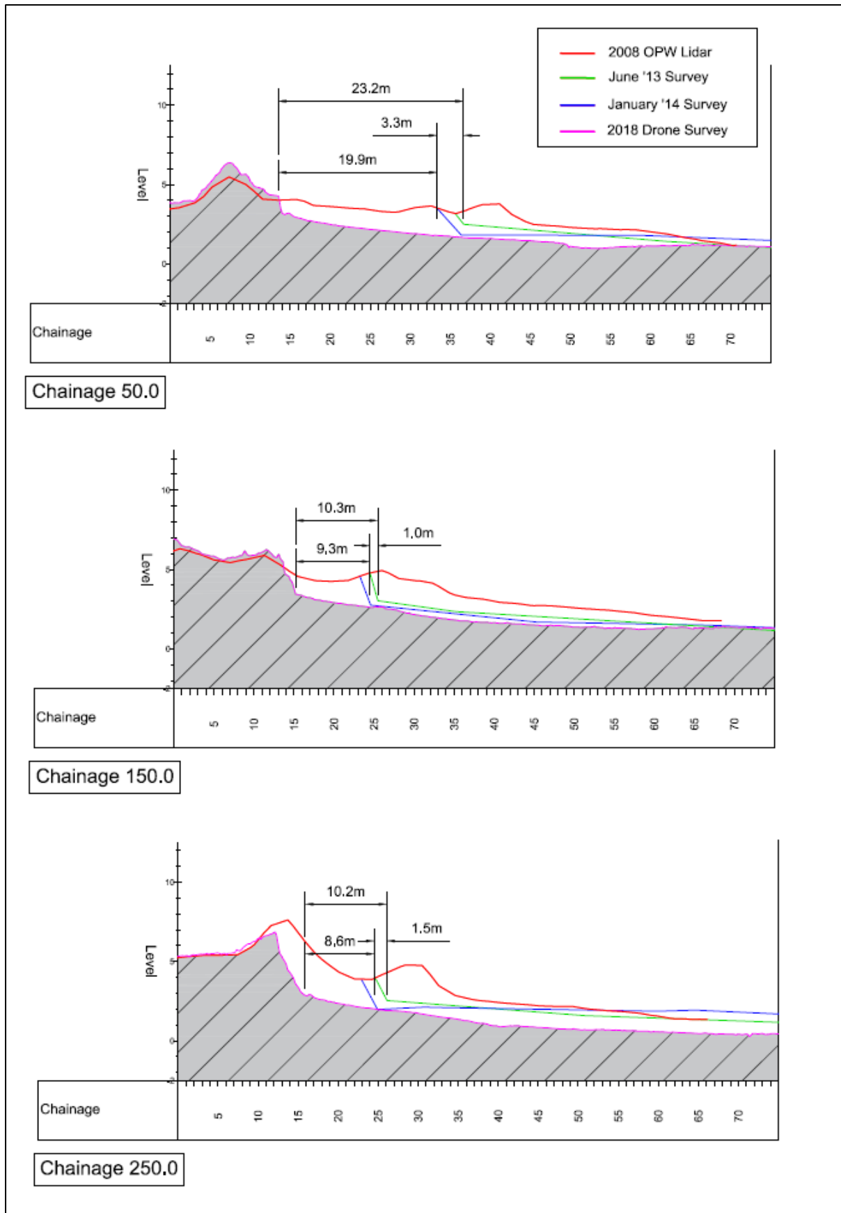
Figure 4.7: Extent of erosion between 2008 – 2018 at representative chainages 50m, 150m and 250m.
