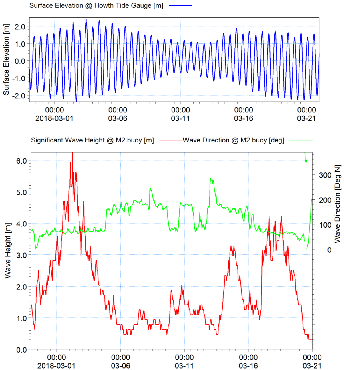
Figure 3.7: Wave climate at M2 buoy and water levels at Howth tide gauge during storm Emma.
