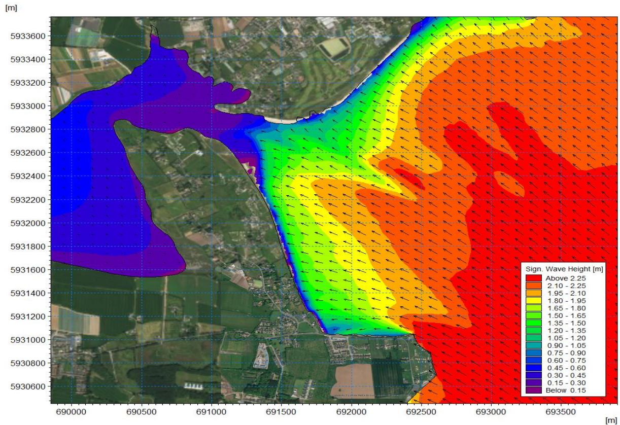
Figure 5.1: Significant wave height and mean wave direction during a joint probability 1 in 50 year return period storm event from the South East.
