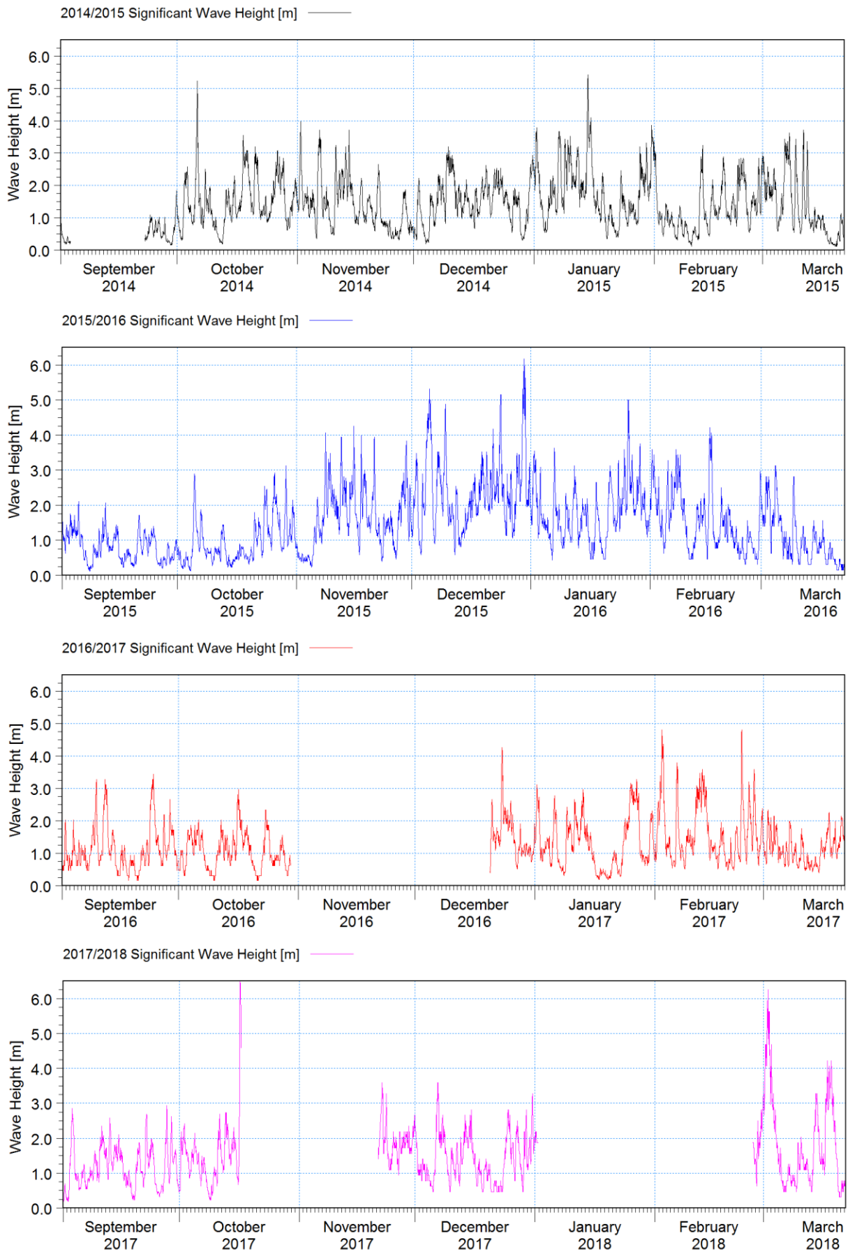
Figure 3.3: Winter wave climate at the M2 buoy from 2014/2015 to 2017/2018.
