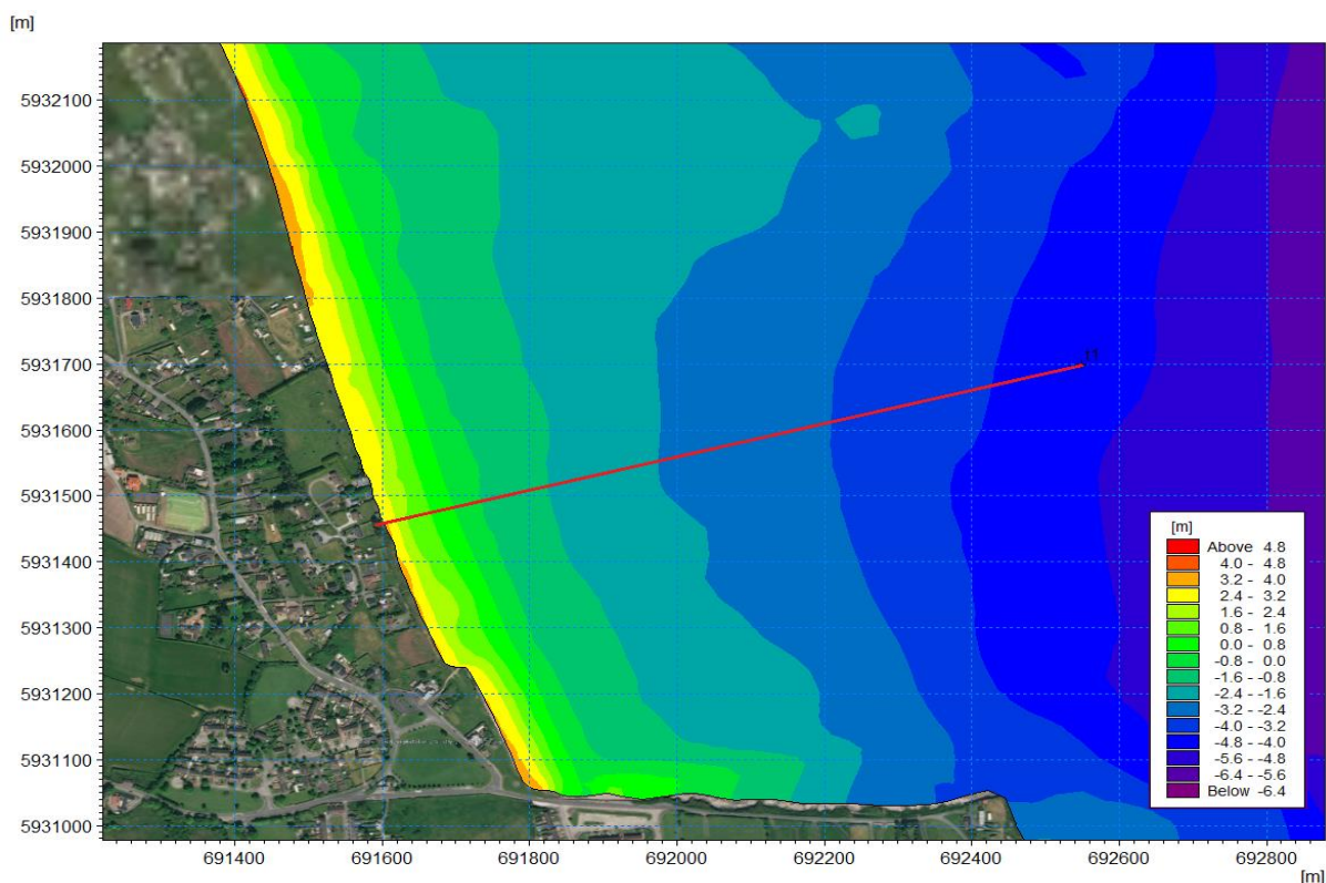
Figure 5.3: Location of the typical cross section profile that was constructed from the 2018 model bathymetry and used in the XBeach morphological modelling simulations.
