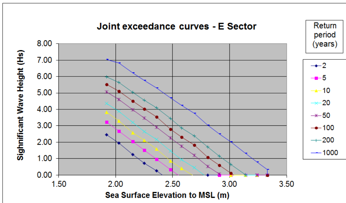
Figure 3.6: Joint Exceedance curves for waves and water levels for the Easterly Sector.
