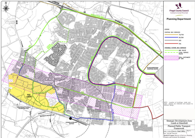
Fig 13.9.2 Existing and Proposed Public Transport Network
